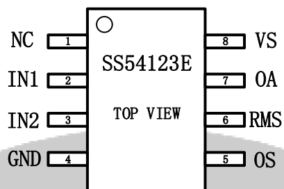
Figure 4. Pin Configuration
